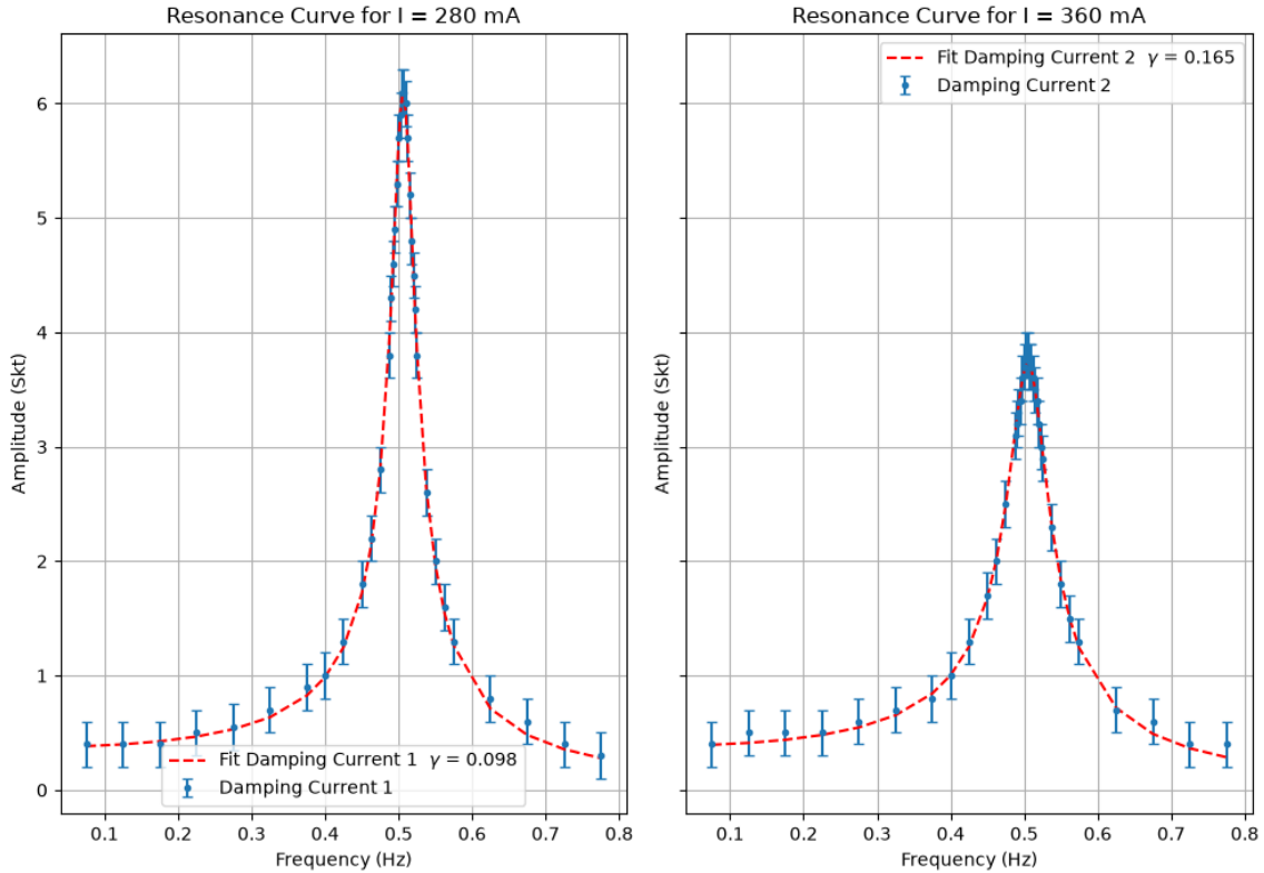
Figure 5.1: Resonance curve for a damping current of 280 mA and 360 mA fitted with the exact brit-wigner function.
